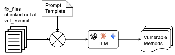
Fig. 1. High-level overview of the vulnerability detection pipeline
