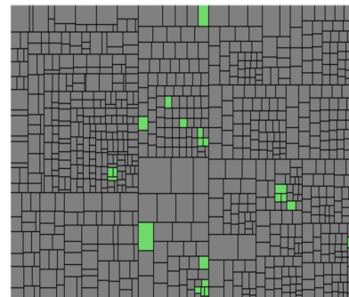
CollectorsTest.testAveragingDouble
