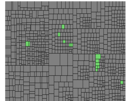
DistinctTest.testDistinctLazy
