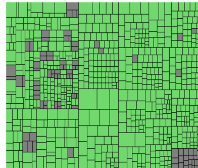
All tests
