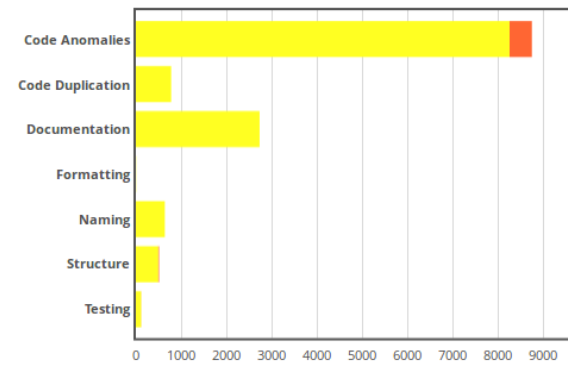
Findings Summary Bar Chart for cqse-all
