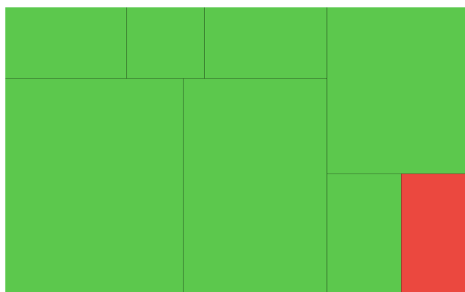
Fig. 8. Issue Test Gaps for TS-15717 after Executing the Impacted Tests Identified by TIA. TGA reveals one remaining test gap.
