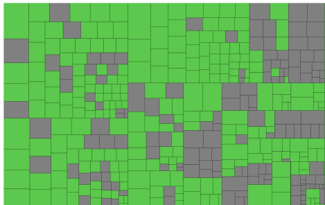
(d) Test Coverage on Method-level. Methods that have been executed are green, all other methods are grey.
