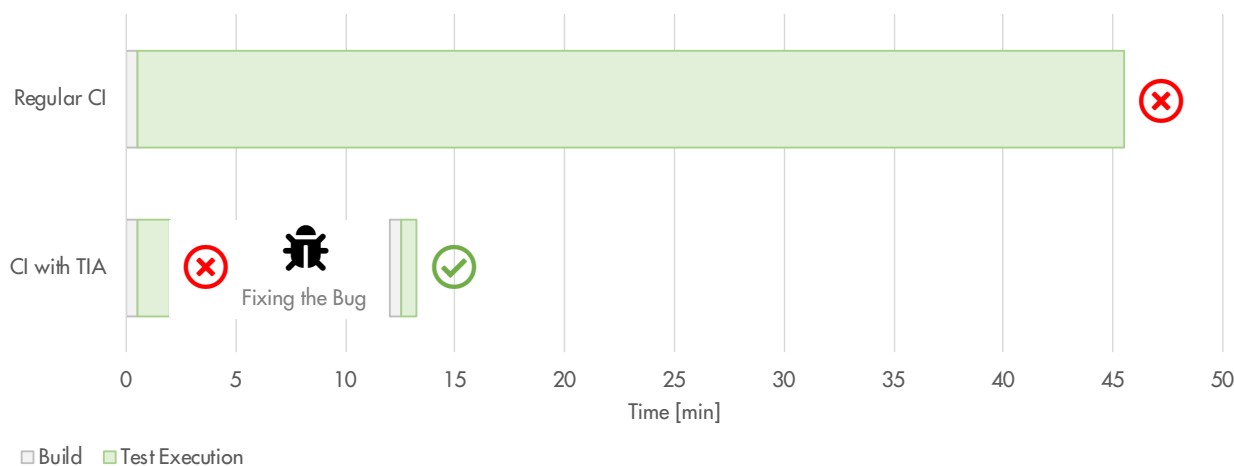
Fig. 7. The Gain from Using Test-Impact Analysis. Two consecutive CI runs using TIA plus correcting a mistake take less time than one CI run with Teamscale’s full test suite.
